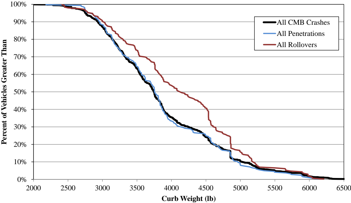
Figure 15. Distribution of Curb Weight in CMB Impacts by Crash Result
